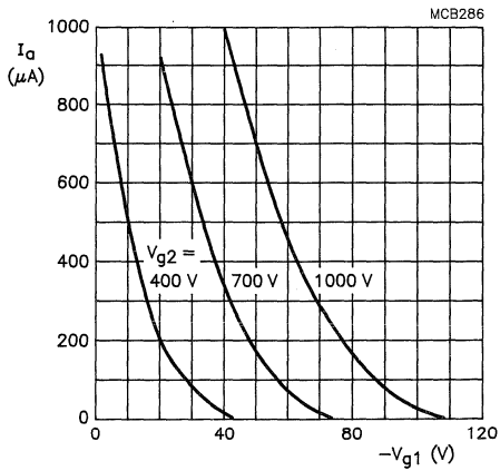
Fig. 4 Anode current as a function of grid 1 voltage. Grid drive; V_{a,g3,g5} = 12 kV.
