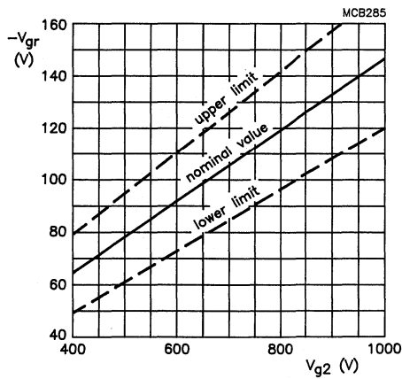
Fig. 6 Limits of grid 1 raster cut-off voltage as a function of grid 2 voltage. Grid drive; V_{a,g3,g5} = 17 kV.
