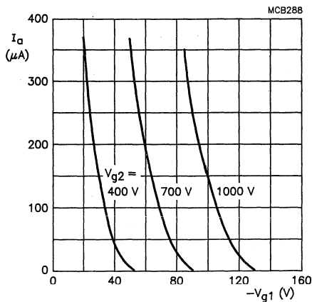
Fig. 4 Anode current as a function of grid 1 voltage. Grid drive; V_{a,g3,g5} = 17 \text{ kV} .
