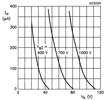
Fig. 3 Anode current as a function of cathode voltage. Cathode drive; V_{a,g3,g5} = 20 kV.
