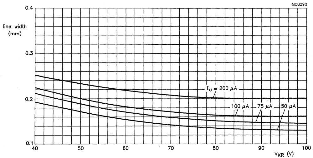
Fig.1 9 inch tube; 90^\circ deflection angle; V_a = 12 kV; raster dimensions 126 mm x 168 mm; 241 active lines at 60 Hz repetition frequency.
