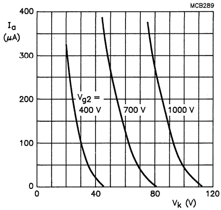
Fig. 1 Anode current as a function of cathode voltage. Cathode drive; V_{a,g3,g5} = (n) \text{ kV}^* .
