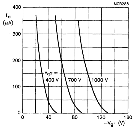
Fig. 4 Anode current as a function of grid 1 voltage. Grid drive; V_{a,g3,g5} = 17 kV.
