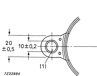
Fig. 13 Tube mounting dimensions; front view.
