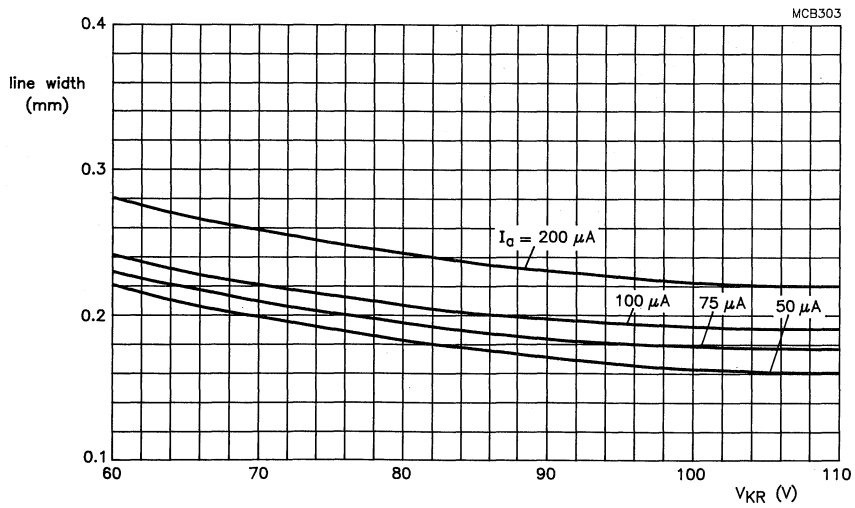
Fig.9 20 inch tube; 110^\circ deflection angle; V_a = 20 kV; raster dimensions 261 mm x 318 mm; 241 active lines at 60 Hz repetition frequency.
