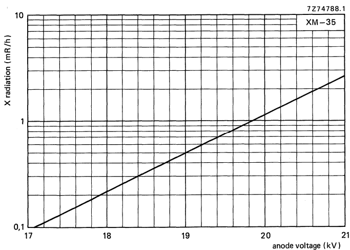
Fig.1 X-radiation limit curve according to JEDEC94, at a constant anode current of 250 \mu\text{A} , measured according TEPAC103A.
