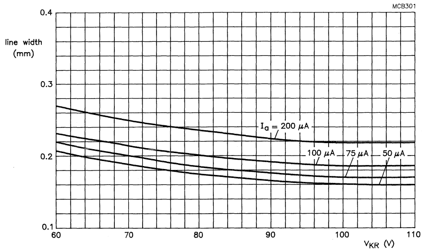
Fig.6 15 inch tube; 110^\circ deflection angle; V_a = 17 kV; raster dimensions 194 mm x 259 mm; 241 active lines at 60 Hz repetition frequency.
