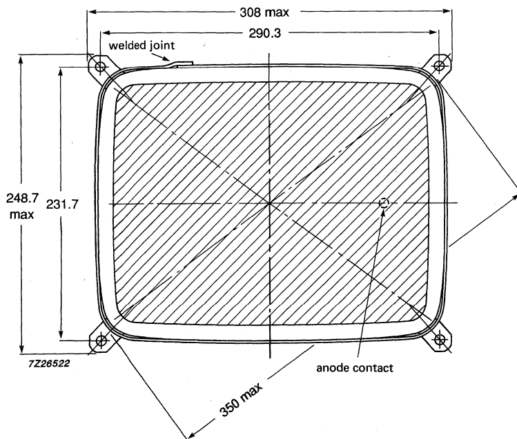
Fig.18 Tube mounting dimensions; front view.
