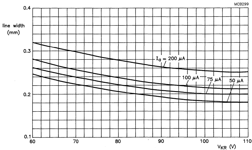
Fig.2 12 inch tube; 90^\circ deflection angle; V_a = 20 kV; raster dimensions 162 mm x 216 mm; 241 active lines at 60 Hz repetition frequency.
