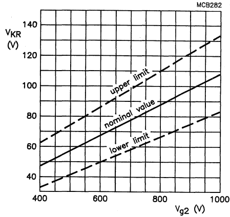
Fig. 5 Limits of cathode cut-off voltage as a function of grid 2 voltage. Cathode drive; V_{a,g3,g5} = 12 \text{ kV} .
