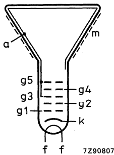
Fig. 11 Electrode configuration.
