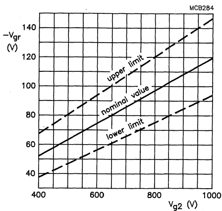
Fig.6 Limits of grid 1 cut-off voltage as a function of grid 2 voltage. Cathode drive; V_{a,g3,g5} = 14 kV.
