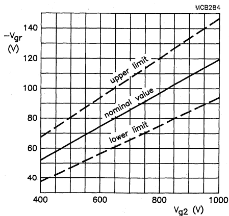
Fig. 6 Limits of grid 1 raster cut-off voltage as a function of grid 2 voltage. Grid drive; V_{a,g3,g5} = 12 kV.
