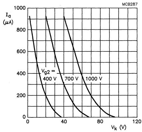
Fig. 3 Anode current as a function of cathode voltage. Cathode drive; V_{a,g3,g5} = 12 \text{ kV} .
