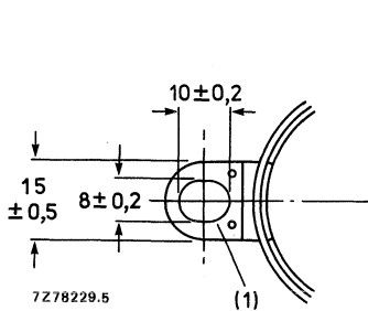
Fig. 13 Tube mounting dimensions; front view.
