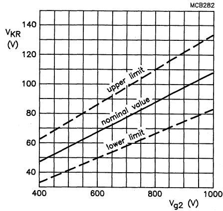
Fig. 5 Limits of cathode cut-off voltage as a function of grid 2 voltage. Cathode drive; V_{a,g3,g5} = 12 kV.
