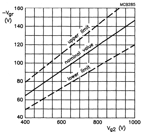
Fig. 6 Limits of grid 1 cut-off voltage as a function of grid 2 voltage. Grid drive; V_{a,g3,g5} = 17 kV.
