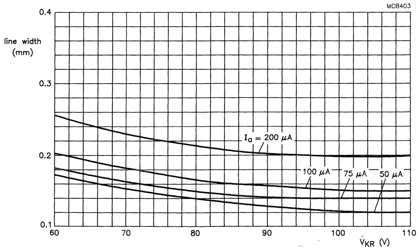
Fig.7 15 inch flat square tube; 110^\circ deflection angle; V_a = 17 kV; raster dimensions 194 mm x 259 mm; 241 active lines at 60 Hz repetition frequency.
