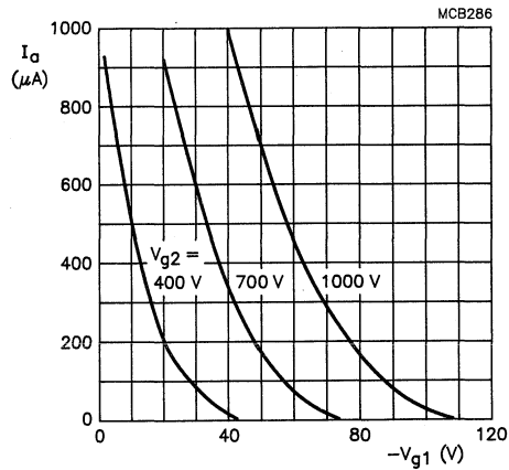
Fig. 4 Anode current as a function of grid 1 voltage. Grid drive; V_{a,g3,g5} = 14 kV.
