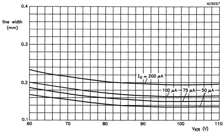
Fig.1 9 inch tube; 90^\circ deflection angle; V_a = 12 kV; raster dimensions 126 mm x 166 mm; 241 active lines at 60 Hz repetition frequency.
