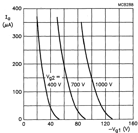
Fig. 4 Anode current as a function of grid 1 voltage. Grid drive; V_{a,g3,g5} = 20 kV.
