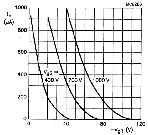
Fig. 2 Anode current as a function of grid 1 voltage. Grid drive; V_{a,g3,g5} = (n) \text{ kV}^* .
