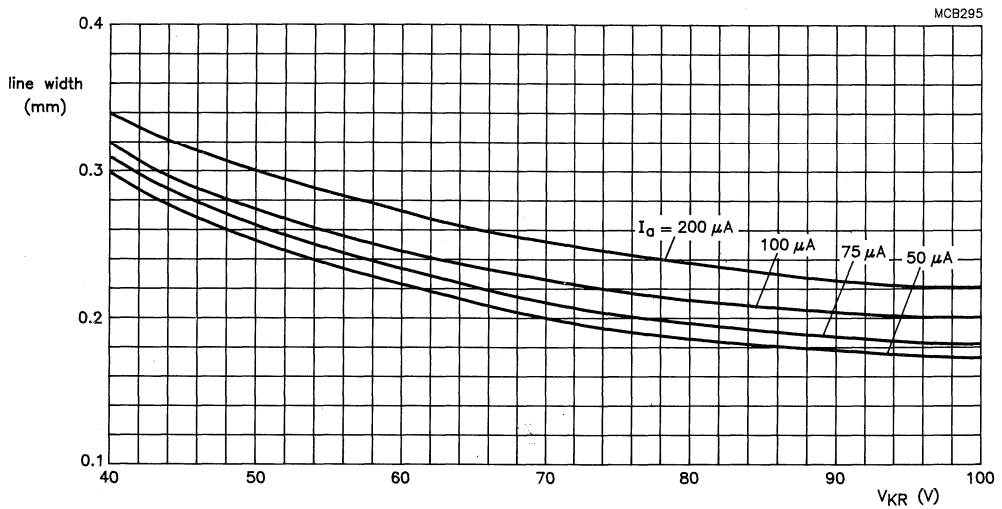
Fig.8 17 inch tube; 110^\circ deflection angle; V_a = 20 kV; raster dimensions 228 mm x 304 mm; 241 active lines at 60 Hz repetition frequency.
