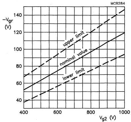
Fig. 6 Limits of grid 1 cut-off voltage as a function of grid 2 voltage. Grid drive; V_{a,g3,g5} = 12 kV.
