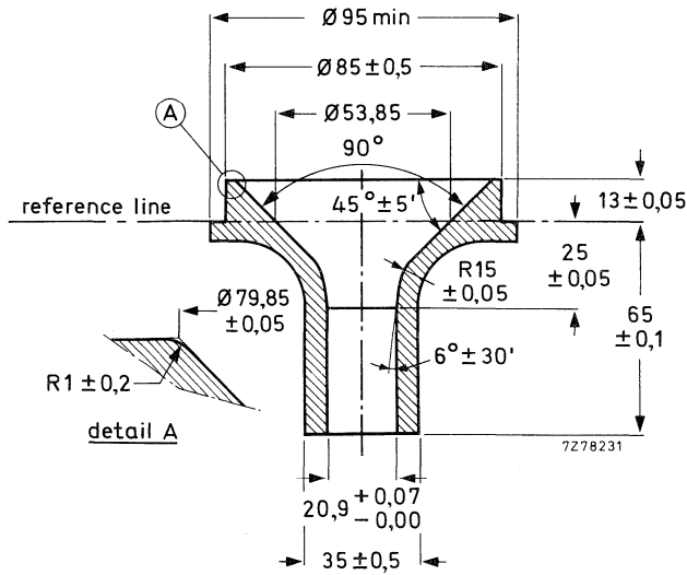
Fig. 2 Reference line gauge for 90° deflection angle.
