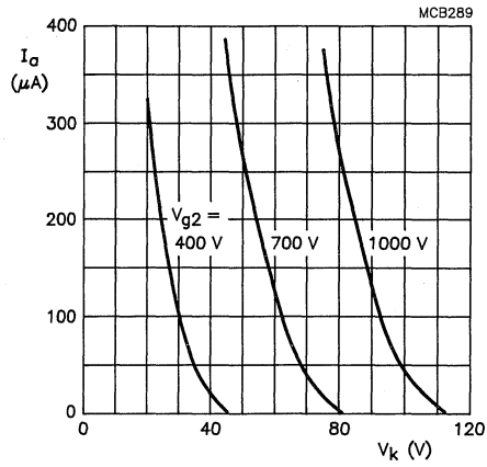
Fig. 3 Anode current as a function of cathode voltage. Cathode drive; V_{a,g3,g5} = 17 kV.
