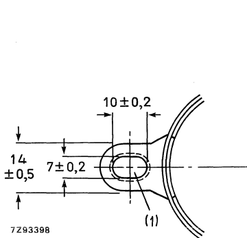
Fig. 19 Tube mounting dimensions; front view.
