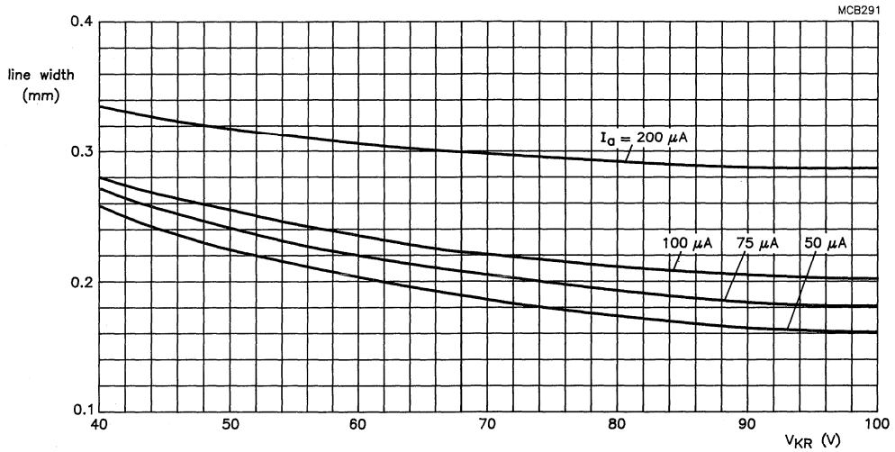
Fig.2 12 inch tube; 90^\circ deflection angle; V_a = 12 kV; raster dimensions 162 mm x 216 mm; 241 active lines at 60 Hz repetition frequency.
