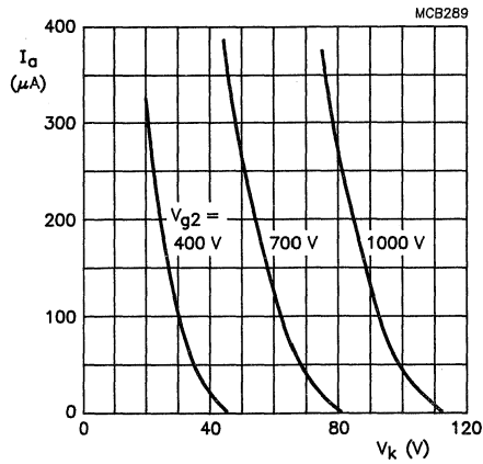
Fig. 3 Anode current as a function of cathode voltage. Cathode drive; V_{a,g3,g5} = 17 \text{ kV} .
