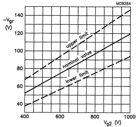
Fig. 6 Limits of grid 1 cut-off voltage as a function of grid 2 voltage. Grid drive; V_{a,g3,g5} = 12 \text{ kV} .
