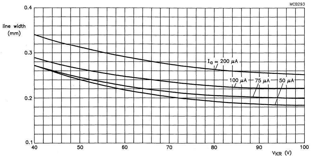
Fig.4 14 inch tube; 90^\circ deflection angle; V_a = 14 kV; raster dimensions 178 mm x 237 mm; 241 active lines at 60 Hz repetition frequency.
