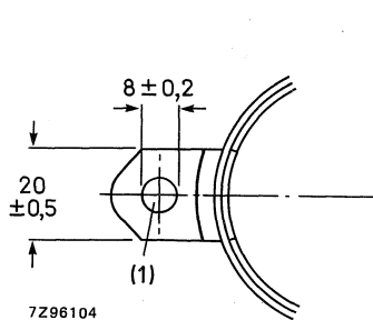
Fig.15 Tube mounting dimensions; front view.
