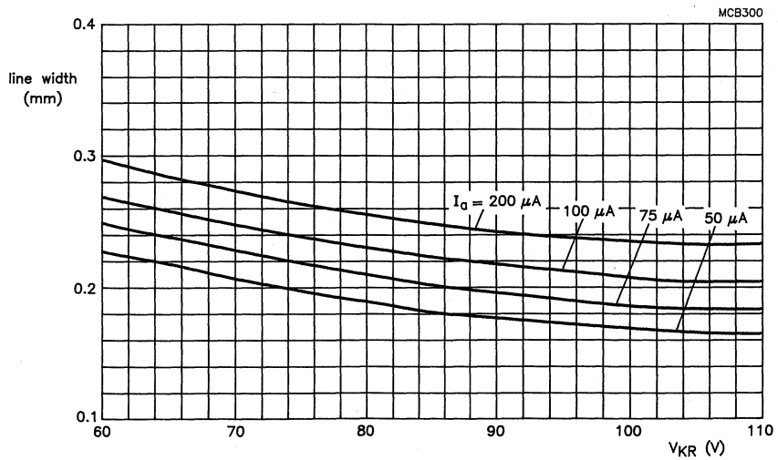
Fig.5 14 inch flat square tube; 90^\circ deflection angle; V_a = 17 kV; raster dimensions 178 mm x 237 mm; 241 active lines at 60 Hz repetition frequency.
