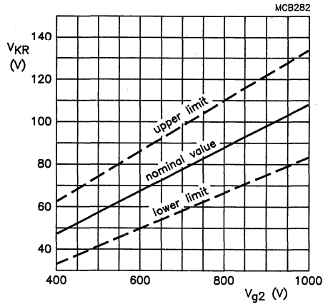
Fig. 5 Limits of cathode cut-off voltage as a function of grid 2 voltage. Cathode drive; V_{a,g3,g5} = 14 kV.
