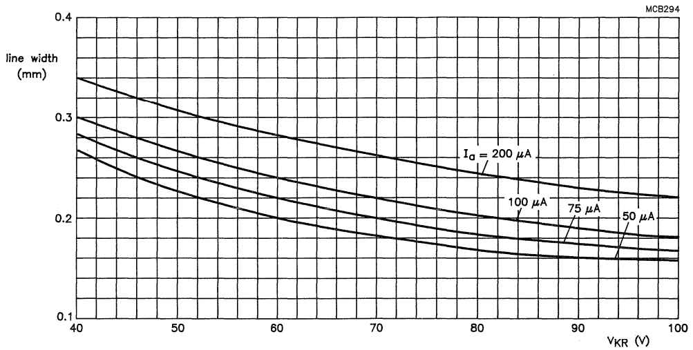
Fig.6 15 inch tube; 110^\circ deflection angle; V_a = 17 kV; raster dimensions 194 mm x 259 mm; 241 active lines at 60 Hz repetition frequency.
