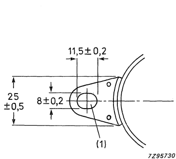
Fig. 25 Tube mounting dimensions; front view.
