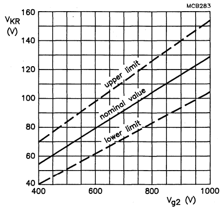
Fig. 5 Limits of cathode raster cut-off voltage as a function of grid 2 voltage. Cathode drive; V_{a,g3,g5} = 20 kV.
