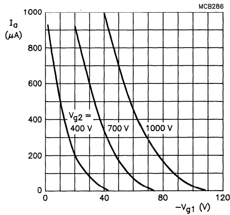
Fig.4 Anode current as a function of grid 1 voltage. Grid drive; V_{a,g3,g5} = 14 kV.
