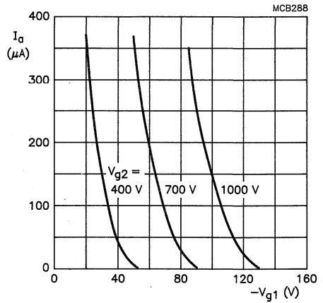
Fig. 2 Anode current as a function of grid 1 voltage. Grid drive; V_{a,g3,g5} = (n) \text{ kV}^* .
