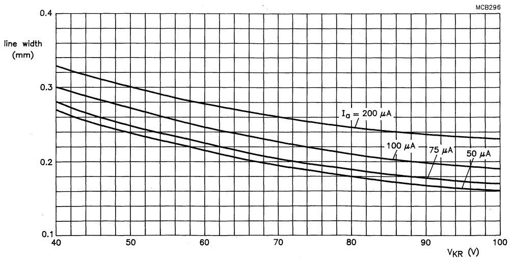
Fig.9 20 inch tube; 110^\circ deflection angle; V_a = 20 kV; raster dimensions 261 mm x 348 mm; 241 active lines at 60 Hz repetition frequency.
