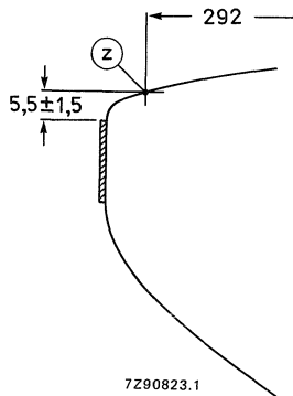
Fig. 20 Rimband position.
