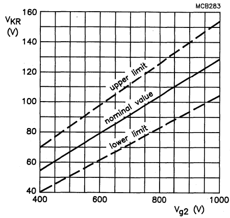
Fig. 5 Limits of cathode raster cut-off voltage as a function of grid 2 voltage. Cathode drive; V_{a,g3,g5} = 17 kV.
