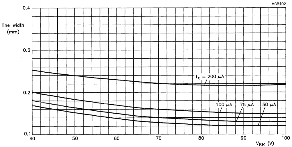
Fig.7 15 inch flat square tube; 110^\circ deflection angle; V_a = 17 kV; raster dimensions 194 mm x 259 mm; 241 active lines at 60 Hz repetition frequency.
