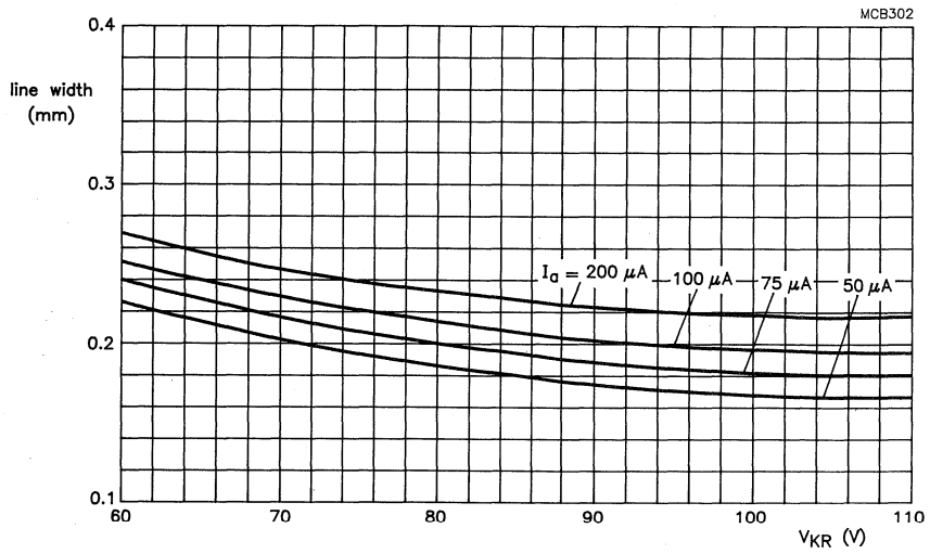
Fig.8 17 inch tube; 110^\circ deflection angle; V_a = 20 kV; raster dimensions 228 mm x 304 mm; 241 active lines at 60 Hz repetition frequency.
