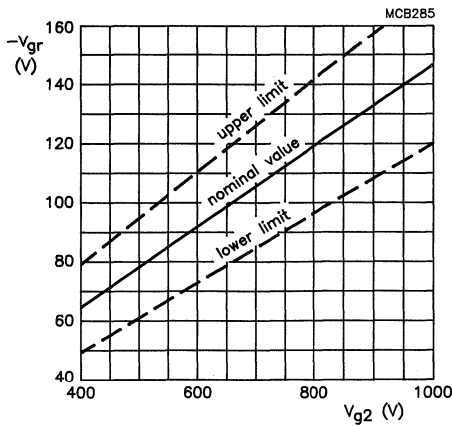
Fig. 6 Limits of grid 1 raster cut-off voltage as a function of grid 2 voltage. Grid drive; V_{a,g3,g5} = 20 kV.
