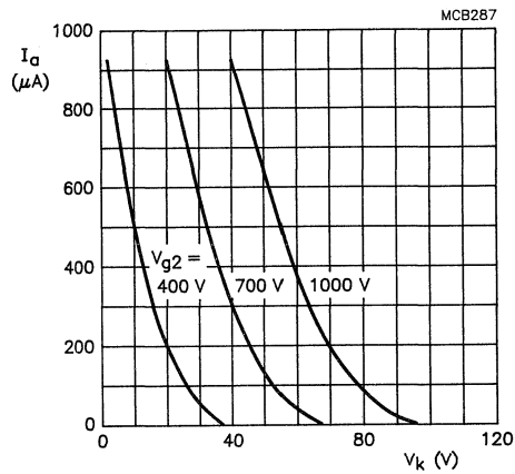
Fig. 3 Anode current as a function of cathode voltage. Cathode drive; V_{a,g3,g5} = 12 kV.
