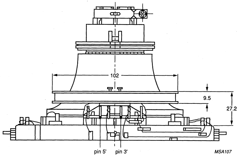
Fig.1 AT1037/AT1039 yoke with optional rotation coil.
