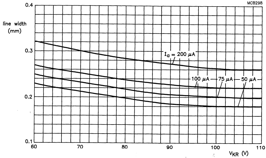
Fig.4 14 inch tube; 90^\circ deflection angle; V_a = 14 kV; raster dimensions 178 mm x 237 mm; 241 active lines at 60 Hz repetition frequency.
