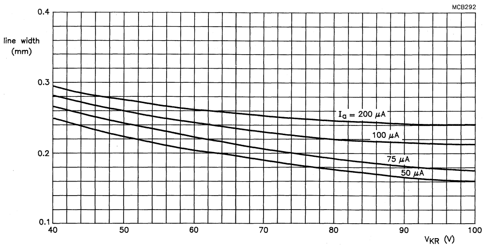
Fig.5 14 inch flat tube; 90^\circ deflection angle; V_a = 14 kV; raster dimensions 178 mm x 237 mm; 241 active lines at 60 Hz repetition frequency.
