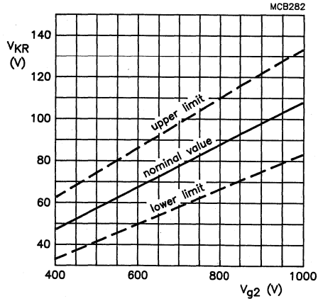
Fig. 5 Limits of cathode raster cut-off voltage as a function of grid 2 voltage. Cathode drive; V_{a,g3,g5} = 12 kV.
