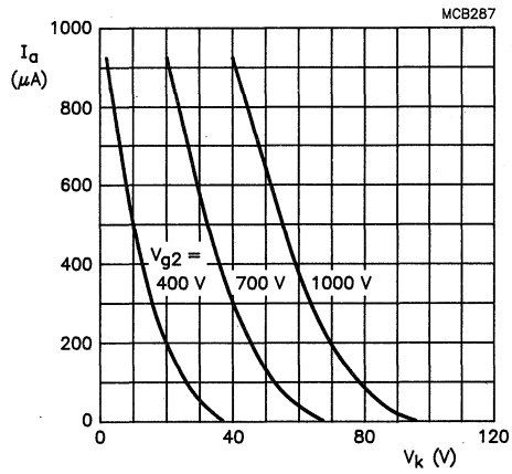
Fig. 1 Anode current as a function of cathode voltage. Cathode drive; V_{a,g3,g5} = (n) \text{ kV}^* .
