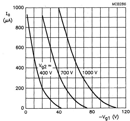
Fig. 4 Anode current as a function of grid 1 voltage. Grid drive; V_{a,g3,g5} = 12 \text{ kV} .
