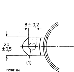
Fig.13 Tube mounting dimensions; front view.
