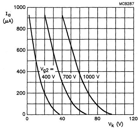
Fig. 3 Anode current as a function of cathode voltage. Cathode drive; V_{a,g3,g5} = 12 kV.
