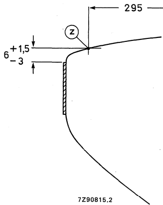
Fig. 19 Tube front view with rimband.
