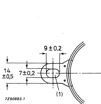
Fig. 24 Tube mounting dimensions; front view.
