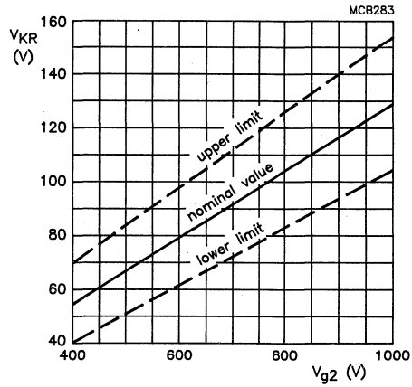
Fig. 5 Limits of cathode cut-off voltage as a function of grid 2 voltage. Cathode drive; V_{a,g3,g5} = 17 kV.
