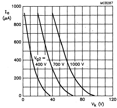
Fig.3 Anode current as a function of cathode voltage. Cathode drive; V_{a,g3,g5} = 14 kV.
