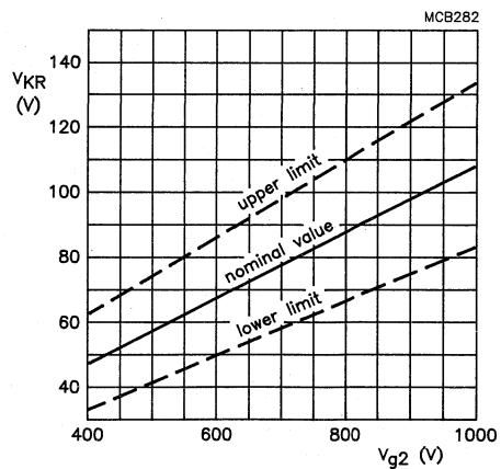
Fig.6 Limits of grid 1 cut-off voltage as a function of grid 2 voltage. Grid drive; V_{a,g3,g5} = 14 kV.
