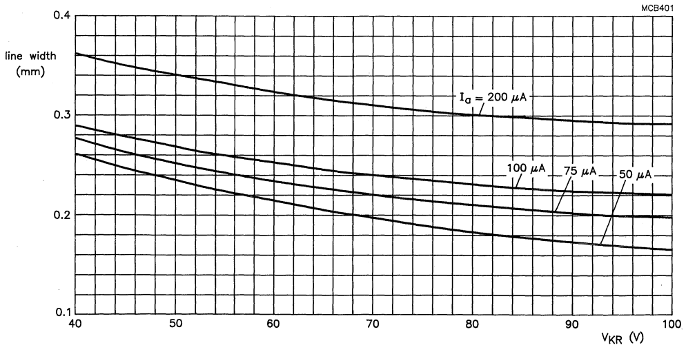
Fig.3 12 inch flat square tube; 90^\circ deflection angle; V_a = 12 kV; raster dimensions 162 mm x 216 mm; 241 active lines at 60 Hz repetition frequency.
