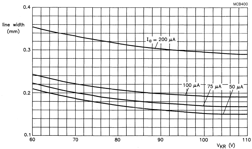
Fig.3 12 inch flat square tubes; 90^\circ deflection angle; V_a = 12 kV; raster dimensions 162 mm x 216 mm; 241 active lines at 60 Hz repetition frequency.
